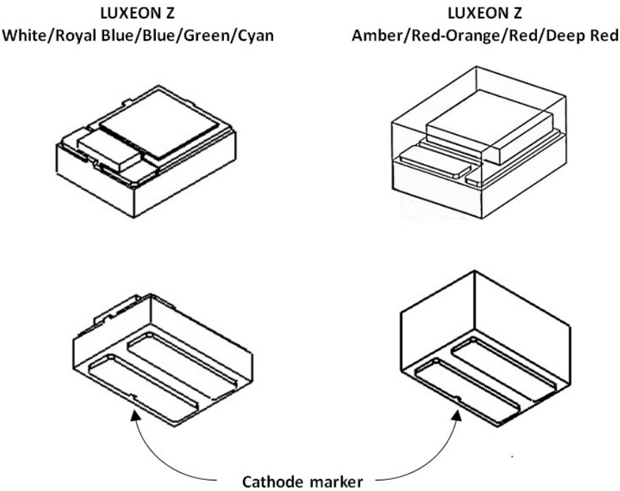
Figure 4. Pad configuration.
