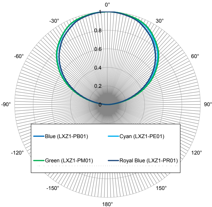
Figure 18. Typical polar radiation pattern for LXZ1-PR01, LXZ1-PB01, LXZ1-PE01 and LXZ1-PM01.
