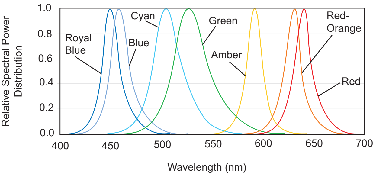
Figure 6. Relative intensity vs. wavelength.
