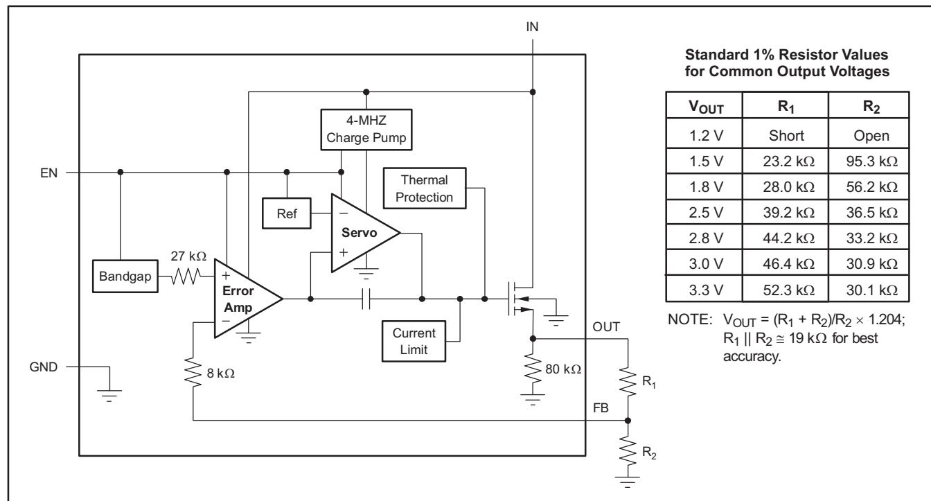
Figure 30. Adjustable-Voltage Version
