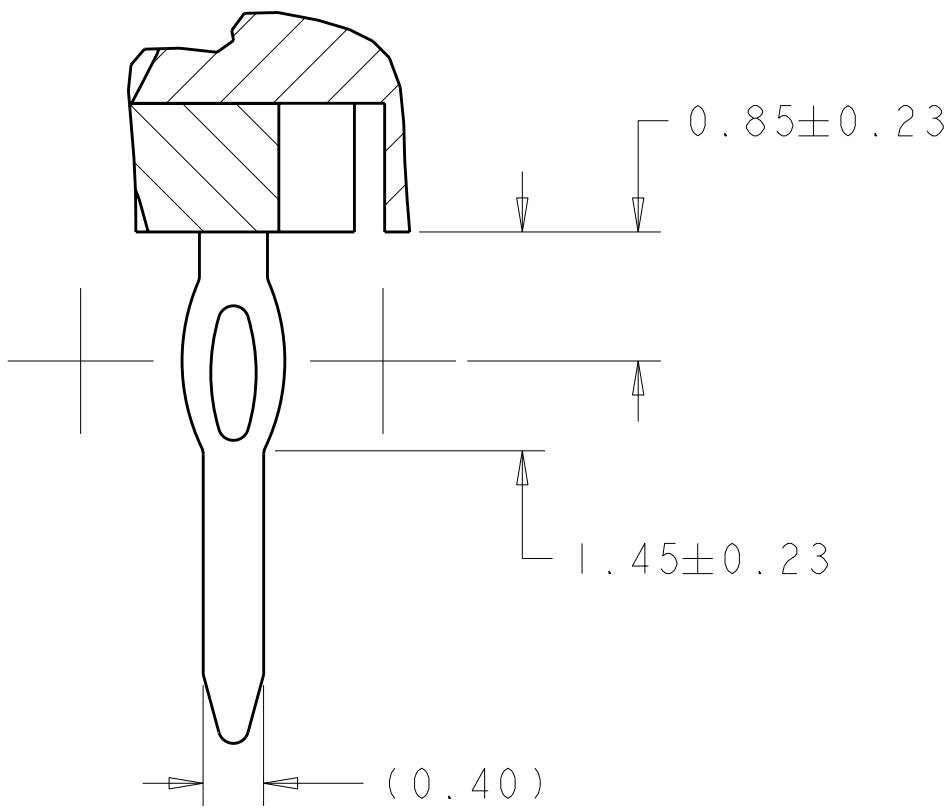
DETAIL H SCALE 20:1
