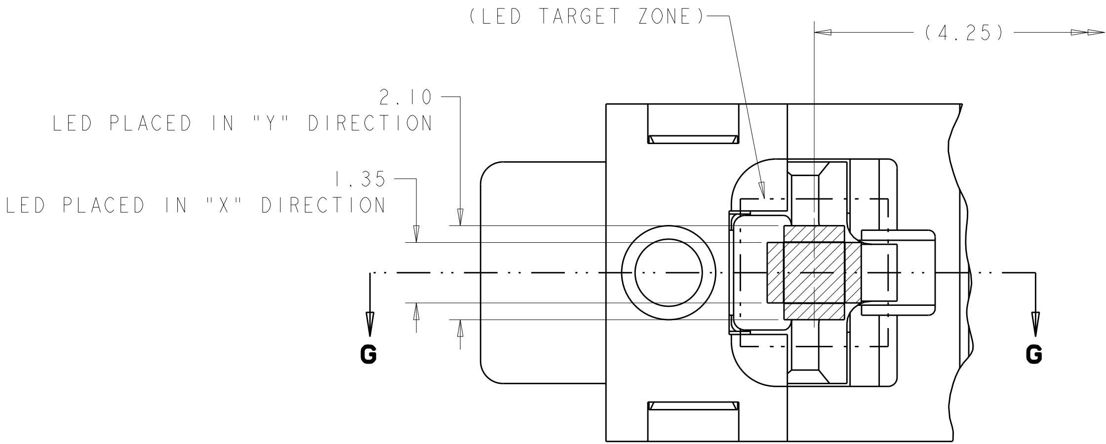
PARTIAL BOTTOM VIEW SCALE 12:1
