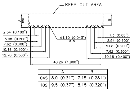
RECOMMENDED P.W.B. PAD LAYOUT
