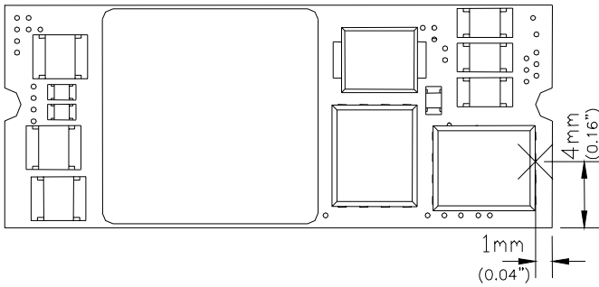
Figure 39: Temperature measurement location
