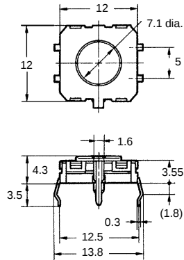
Flat Plunger Type (with Ground Terminal) B3W-4100, -4105
