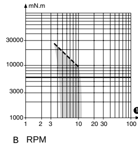
Nominal speed and torque curves 82 802 5
