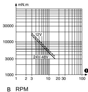
Nominal speed and torque curves 82 812 5
