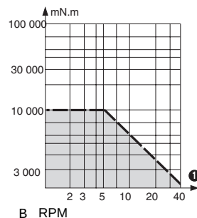
Nominal speed and torque curves 80 814 0
