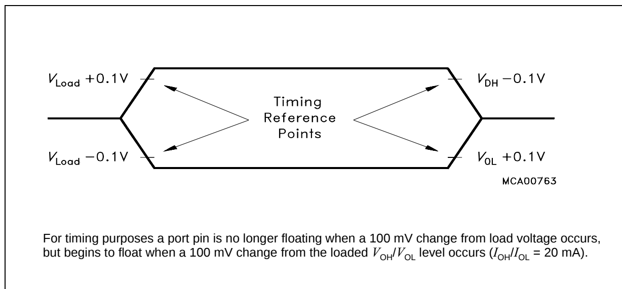
Figure 15 Float Waveforms
