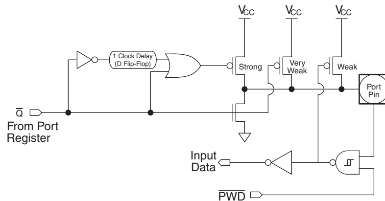
Figure 15-1. Quasi-bidirectional Output
