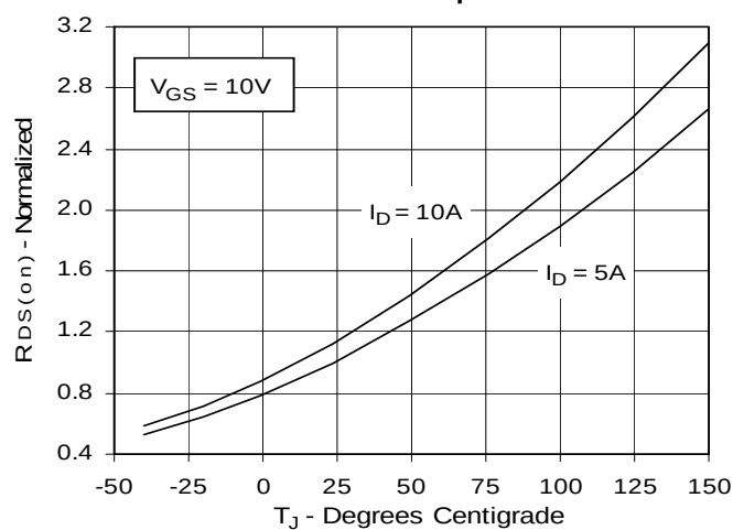
Fig. 5. R_{DS(on)} Normalized to 0.5 I_{D25} Value vs. Junction Temperature
