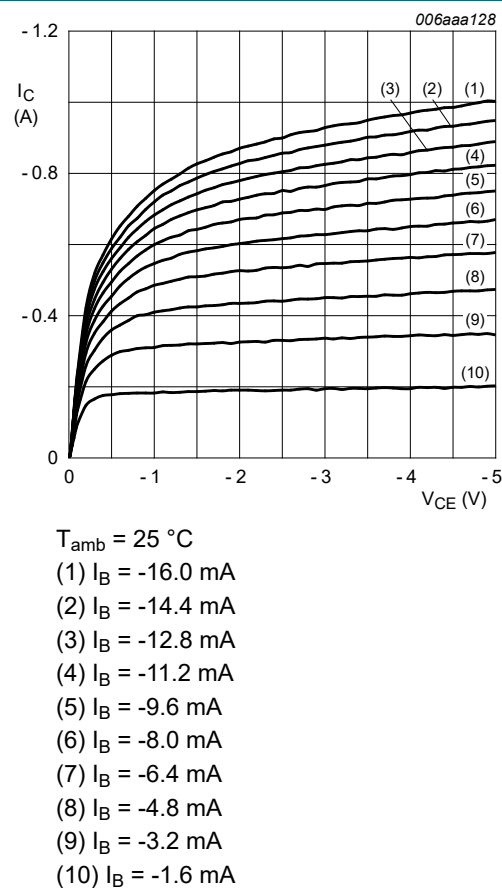
Fig. 7. BC807-16: Collector current as a function of collector-emitter voltage; typical values
