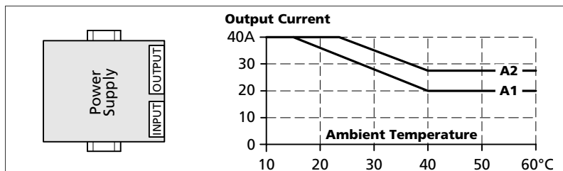
Fig. 25-16 Mounting Orientation E (Horizontal ccw)
