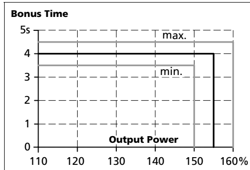
Fig. 6-3 Bonus time vs. output power
