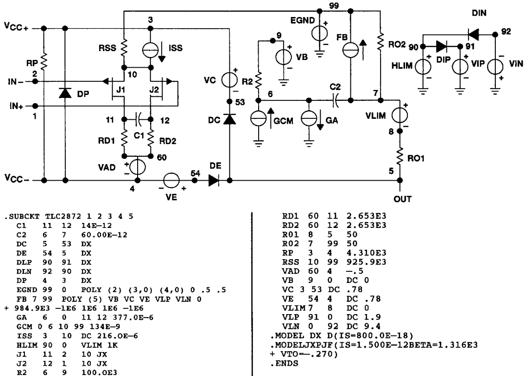
Figure 20. Boyle Macromodel and Subcircuit
