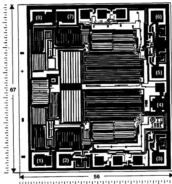
BONDING PAD ASSIGNMENTS
