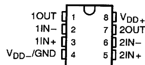
D OR P PACKAGE (TOP VIEW)
