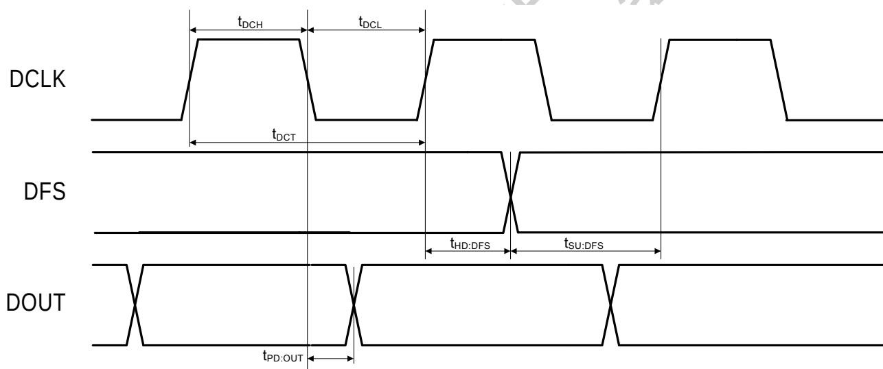
Figure 6. Digital Audio Interface Timing Parameters, I²S Mode
