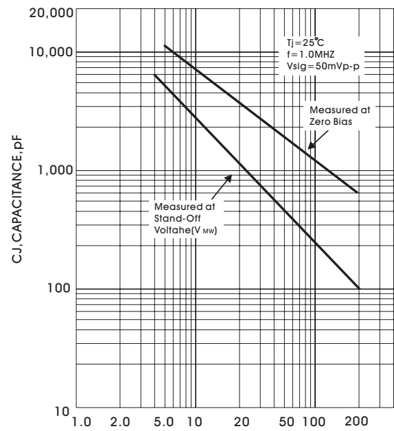
FIGURE 4 TYPICAL CAPACITANCE
