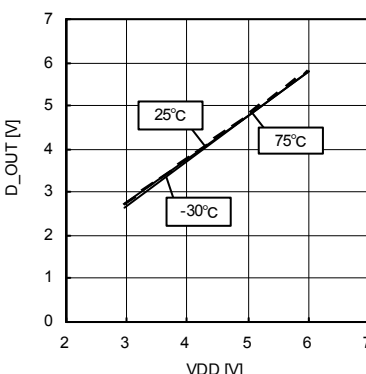
Fig.18 D_OUT Output High Voltage (source 1mA)
