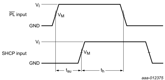
Fig 13. Set-up times for (PL) input to (SHCP) input
