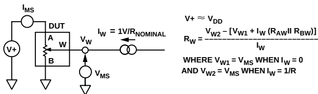
Figure 28. Wiper Resistance Test Circuit
