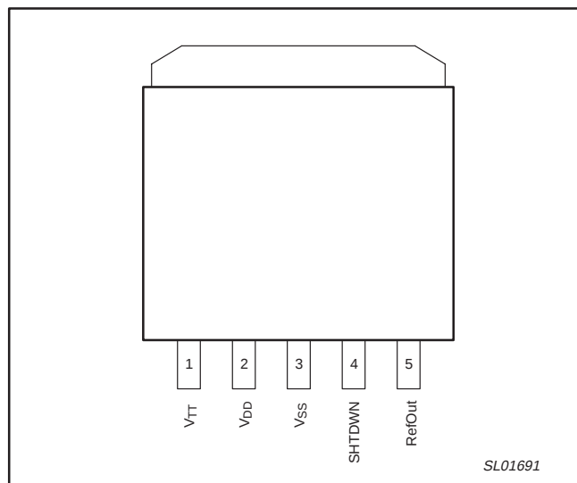
Figure 2. Pin configuration.
