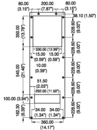
Drilling Template
