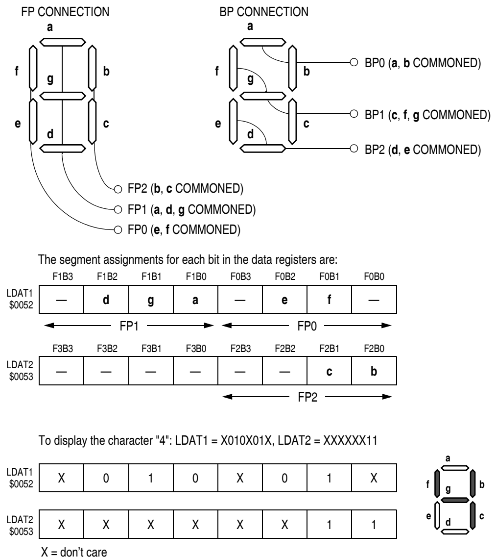
Figure 17-12. 7-Segment Display Example
