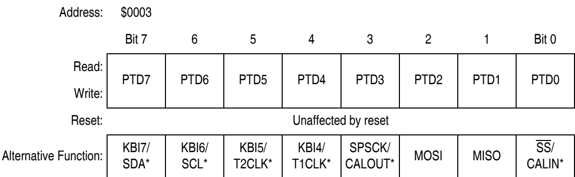
Figure 18-13. Port D Data Register (PTD)
