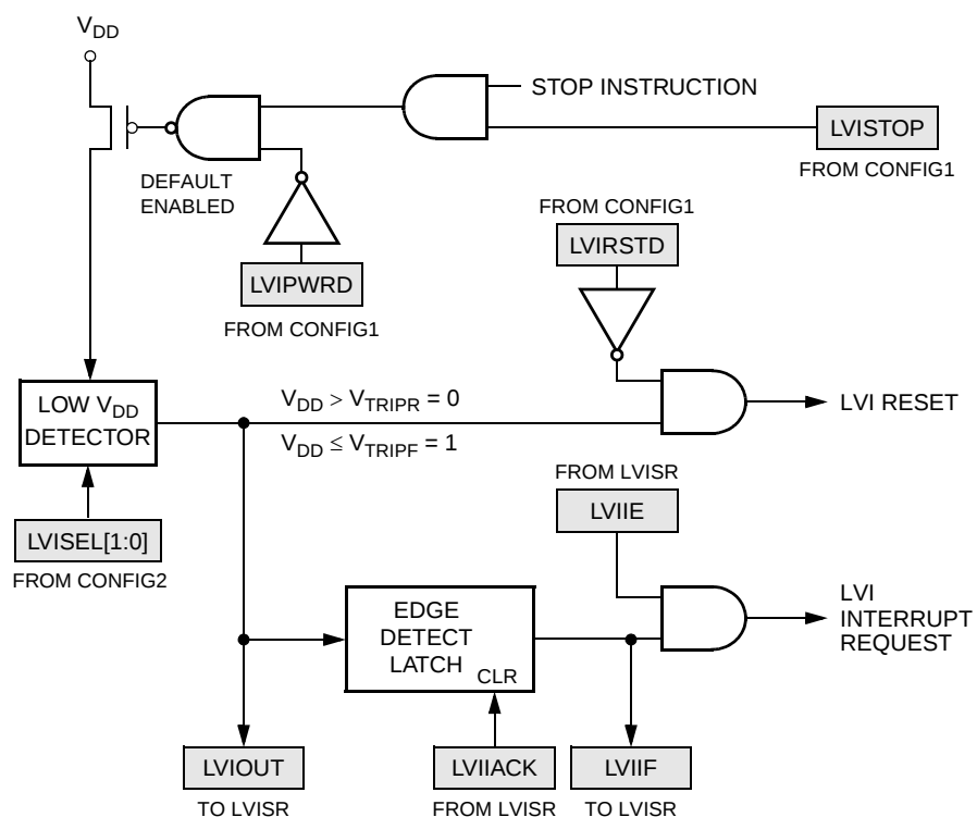
Figure 22-2. LVI Module Block Diagram
