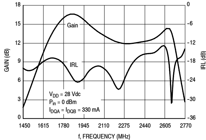
Figure 27. Broadband Frequency Response
