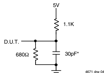
Figure 2. Output Load
