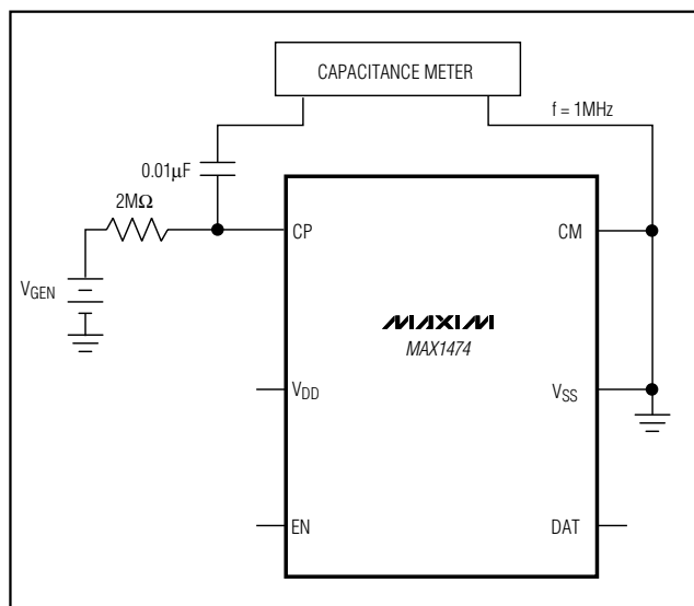
Figure 3a. Capacitance vs. Voltage (Single Ended)
