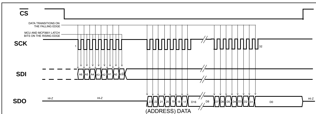
FIGURE 6-4: Device Read (SPI Mode 1,1 - Clock Idles High).
