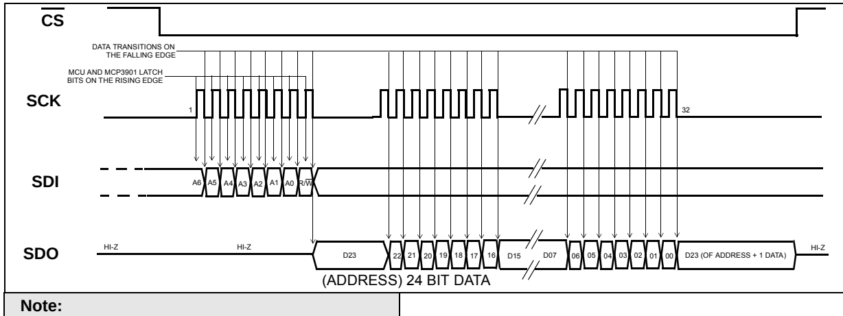
FIGURE 6-2: Device Read (SPI MODE 0,0 - Clock Idles Low).
