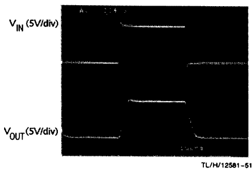
FIGURE 2. The LM6172 Driving a 510 pF Load with a 30 \Omega Isolation Resistor
