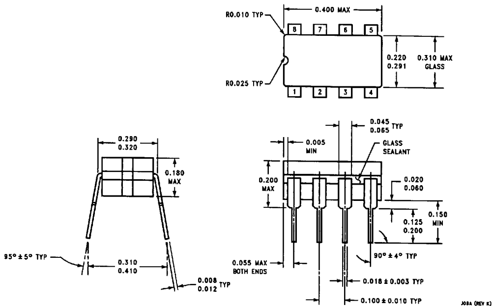
8-Lead Ceramic Dual-In-Line Package Order Number LM6172AMJ-QML or 5962-9560401QPA NS Package Number J08A
