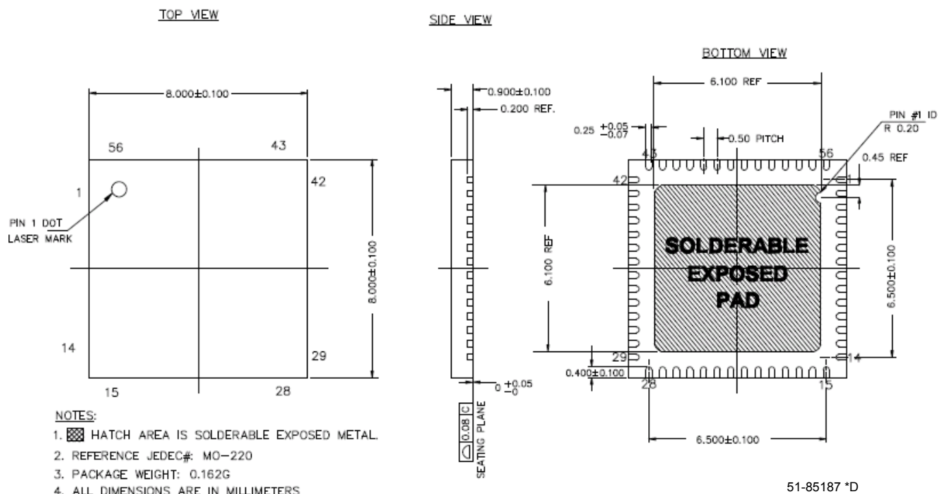
Figure 8. 56-Pin Sawn QFN (8X8X1.0 mm)
