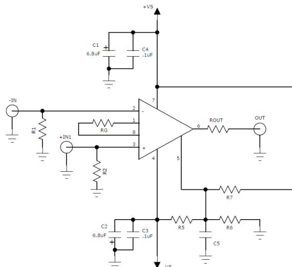
Figure 6. CEB024 Schematic
