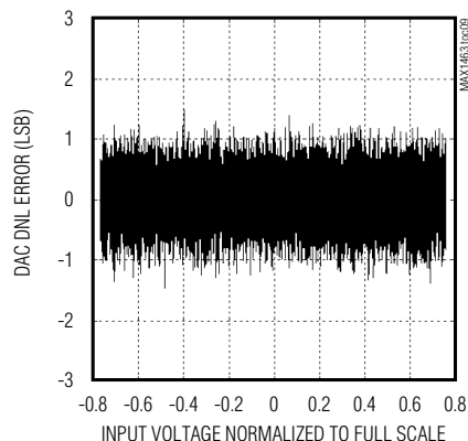
DAC DNL
