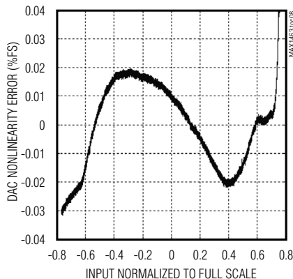
DAC INL
