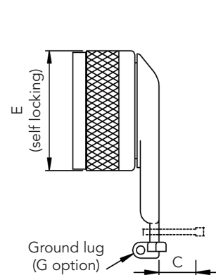
90° plastic collar Type 55
