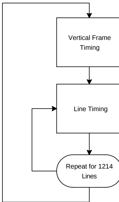
Figure 20. Progressive Scan Flow Chart
