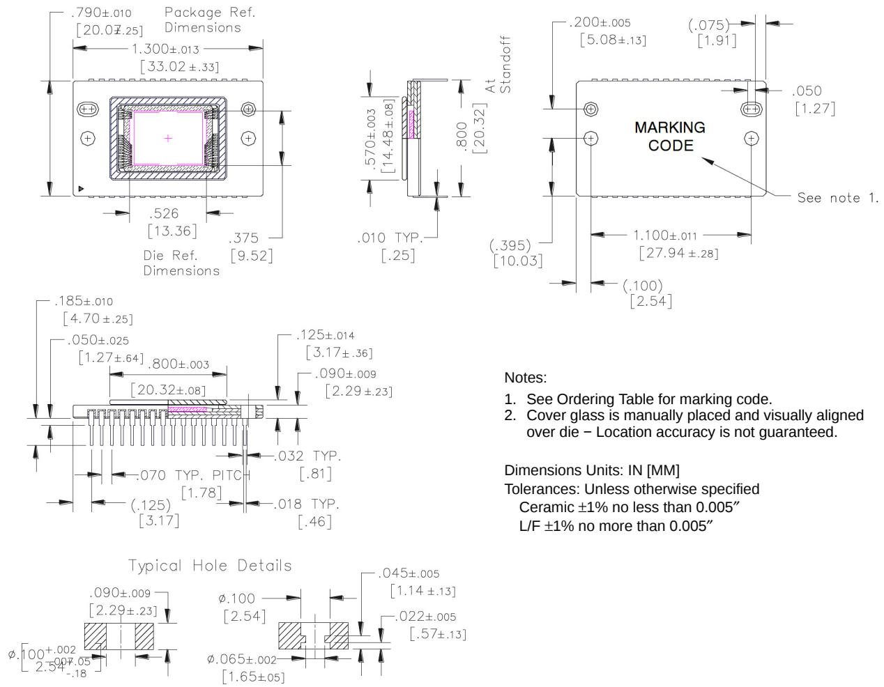
Figure 36. Completed Assembly
