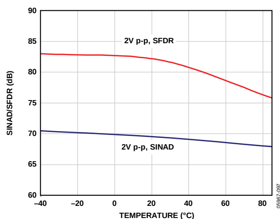
Figure 44. SINAD/SFDR vs. Temperature, f_{IN} = 19.7 MHz, AD9222-65
