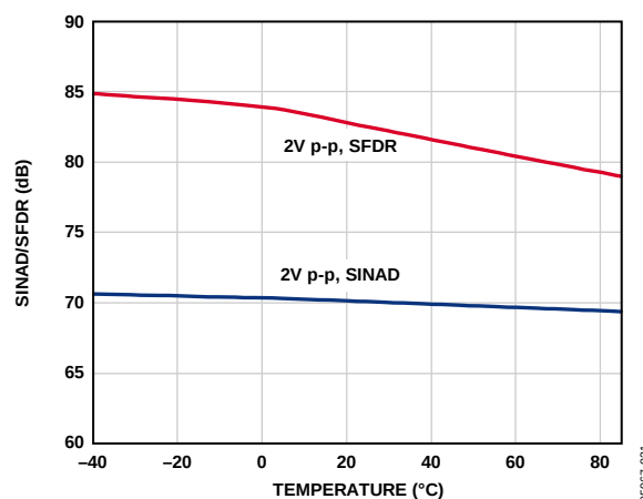
Figure 43. SINAD/SFDR vs. Temperature, f_{IN} = 20.1 MHz, AD9222-50
