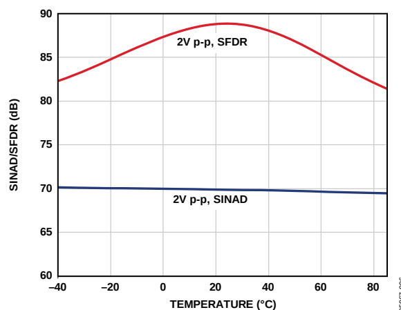
Figure 42. SINAD/SFDR vs. Temperature, f_{IN} = 2.3 MHz, AD9222-65
