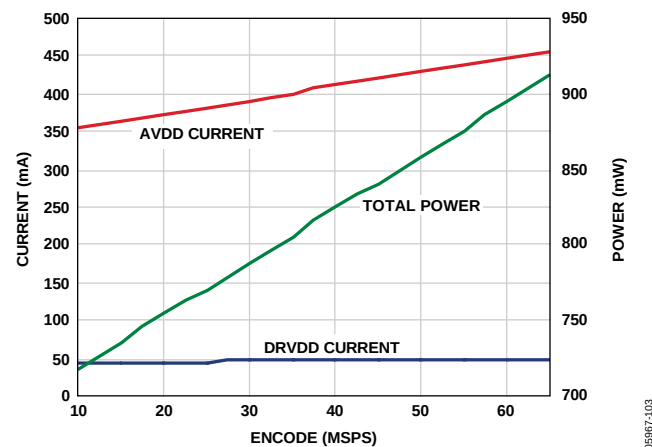
Figure 70. Supply Current vs. f_{\text{SAMPLE}} for f_{\text{IN}} = 10.3 \text{ MHz} , AD9222- 65
