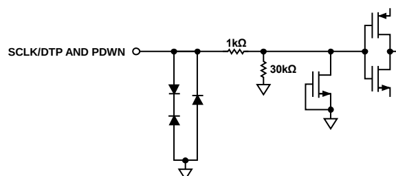
Figure 10. Equivalent SCLK/DTP and PDWN Input Circuit
