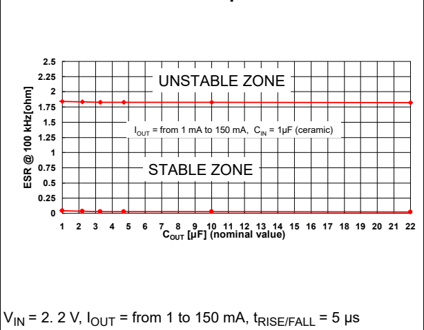
Figure 35. ESR required for stability with ceramics capacitors
