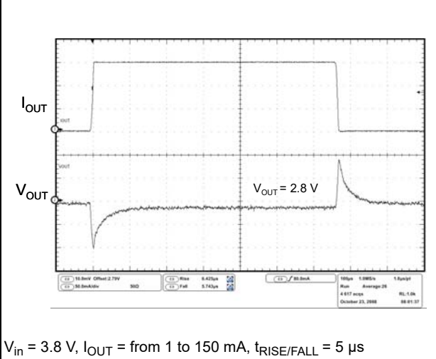
Figure 34. Load transient ( V_{OUT} = 2.8\text{ V} )
