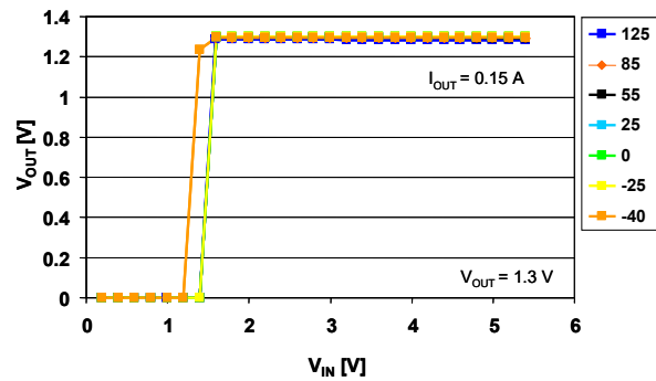
Figure 11. Output voltage vs. input voltage ( V_{OUT} = 1.3 V )
