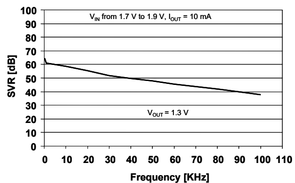
Figure 25. Supply voltage rejection vs. frequency ( V_{OUT} = 1.3\text{ V} )
