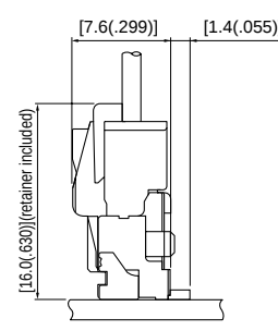
PA Receptacle + PA Header (Retainer mountable type)
