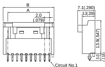
(10 to 12, 15 circuits)
