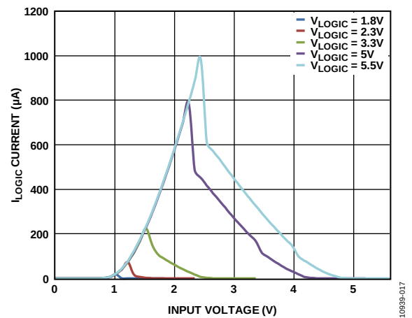
Figure 17. I_{\text{LOGIC}} Current vs. Digital Input Voltage
