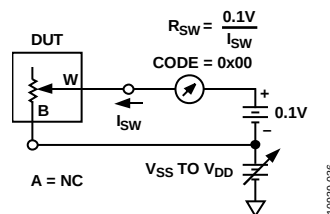
Figure 36. Incremental On Resistance
