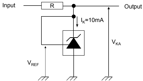
Figure 6. Test circuit V_{KA} = V_{REF}
