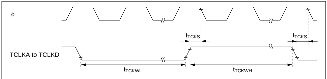
Figure 21.25 TPU Clock Input Timing
