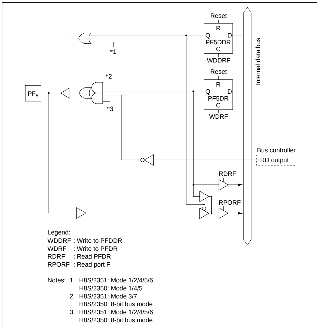
Figure C.12 (f) Port F Block Diagram (Pin PF 5 )
