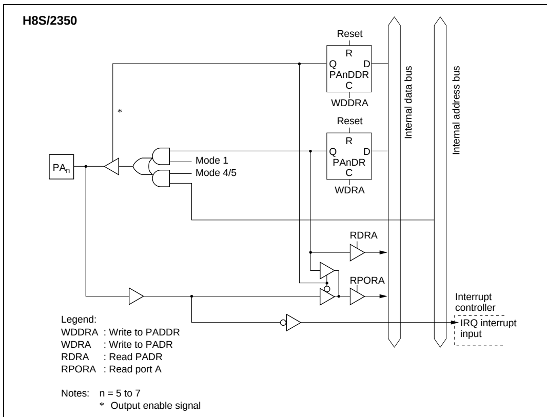
Figure C.7 (c-2) H8S/2350 Port A Block Diagram (Pins PA 5 to PA 7 )
