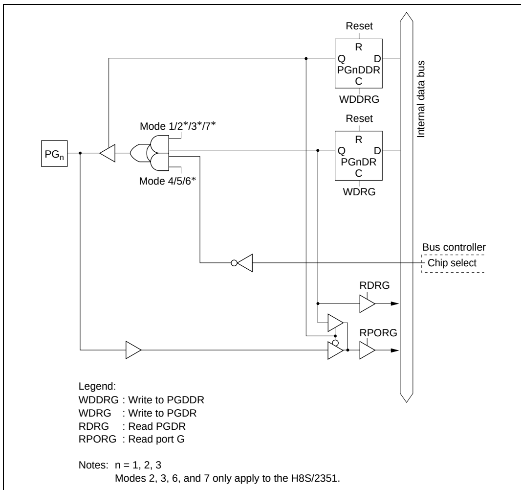
Figure C.13 (b) Port G Block Diagram (Pins PG_1 to PG_3 )
