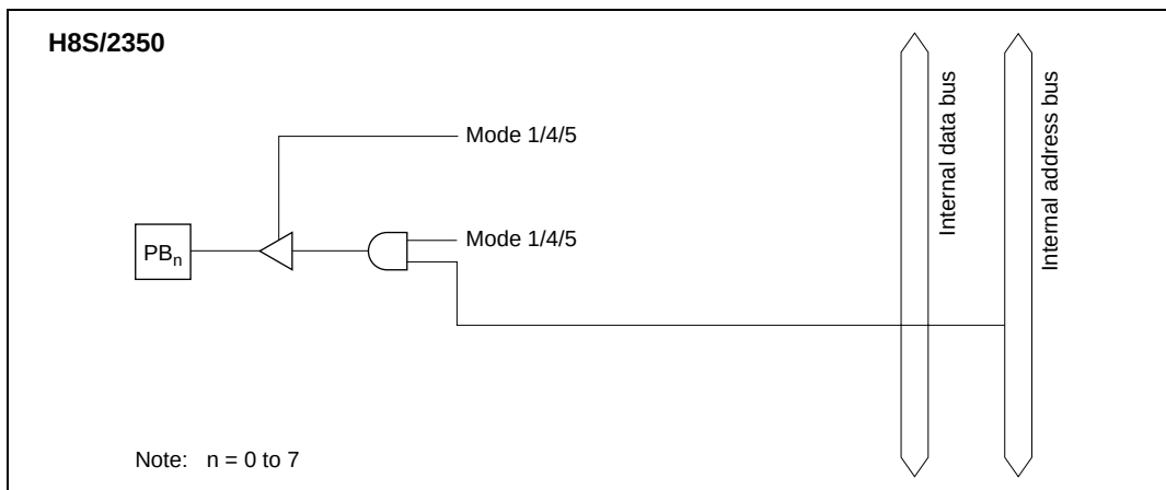
Figure C.8 (b) H8S/2350 Port B Block Diagram (Pin PB_n )
