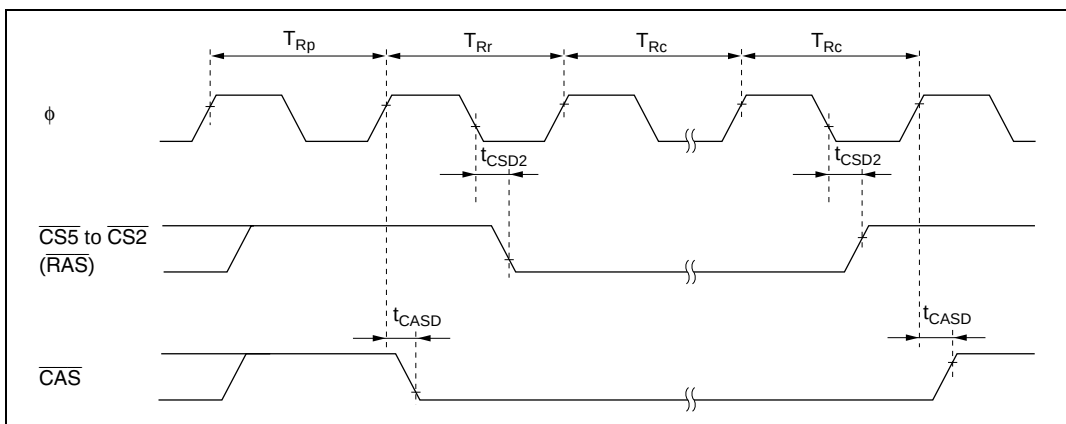
Figure 21.13 Self-Refresh Timing
