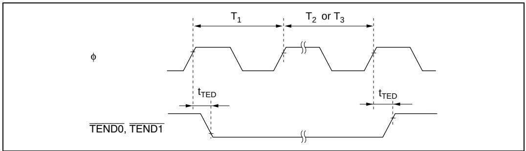
Figure 21.20 DMAC \overline{\text{TEND}} Output Timing
