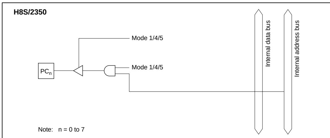
Figure C.9 (b) H8S/2350 Port C Block Diagram (Pin PC_n )
