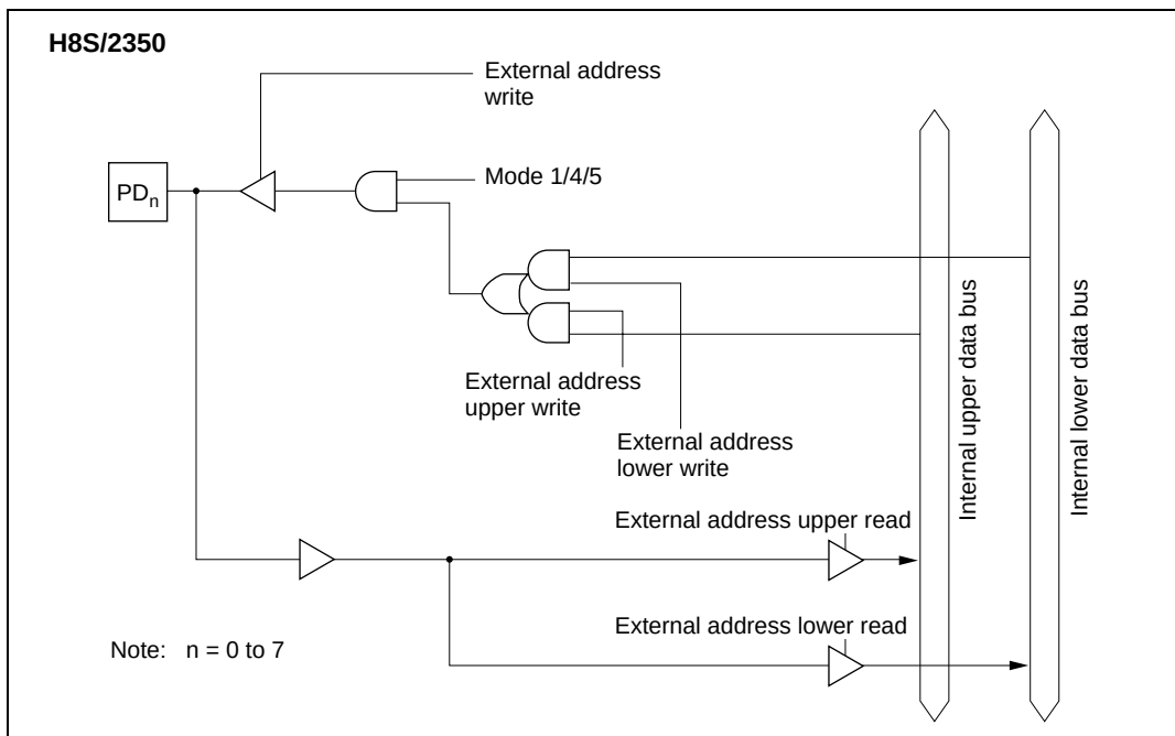
Figure C.10 (b) H8S/2350 Port D Block Diagram (Pin PD_n )
