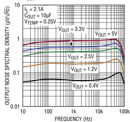
Output Noise Spectral Density, C_{SET} = 0
