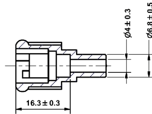
B-B SECTIONAL:
