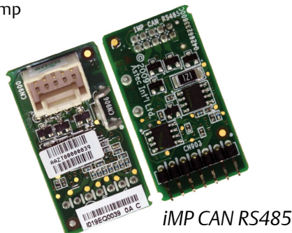
RS485/CAN - to - I2C
