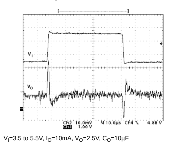
Figure 19. Line transient
