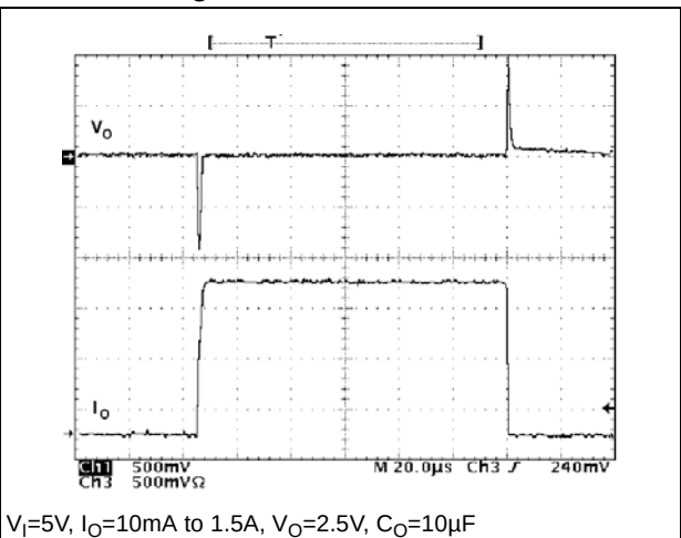
Figure 20. Load transient
