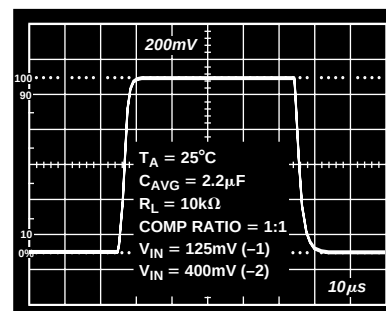
TPC 8. Large Signal Transient Response
