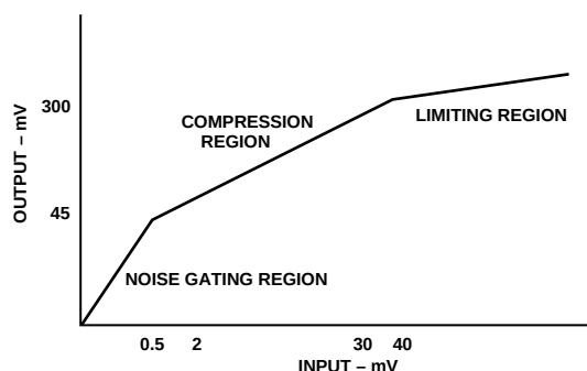
Figure 10. Transfer Characteristic
