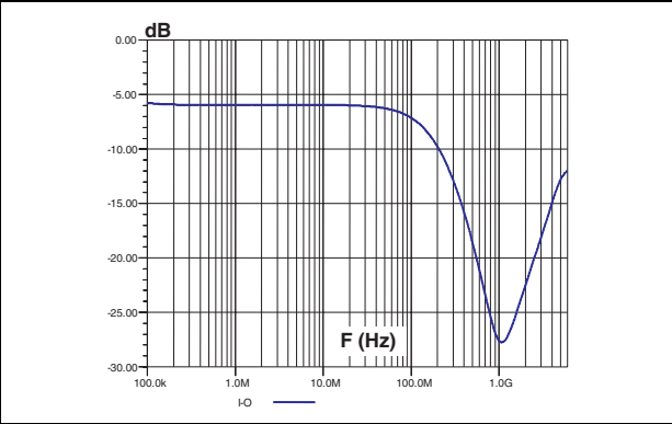
Figure 4. S21 attenuation measurement ( V_{bias} = 0\text{ V} )
