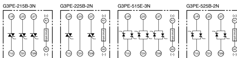
Terminal Arrangement/Internal Circuit Diagram
