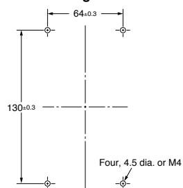
Mounting Holes
