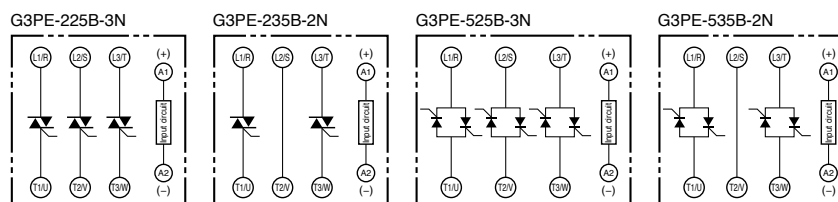
Terminal Arrangement/Internal Circuit Diagram
