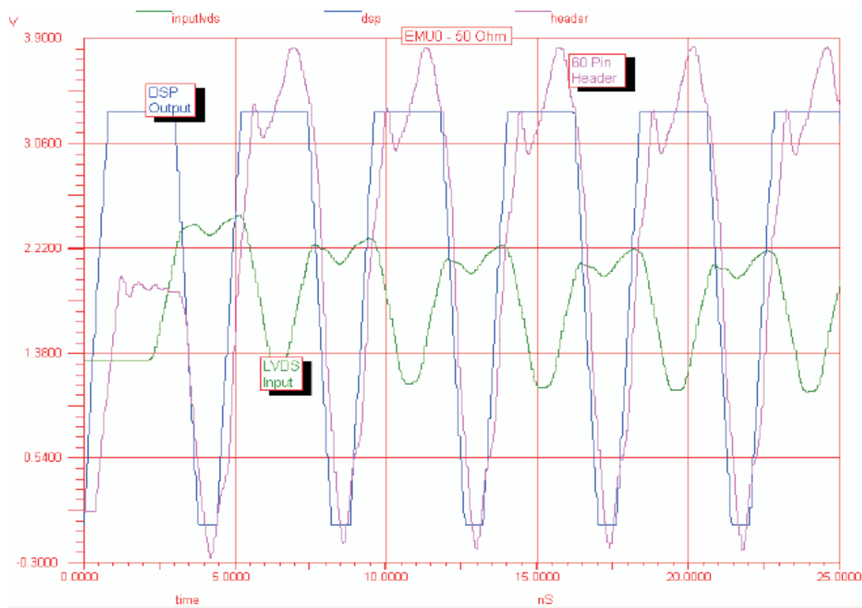
Figure 34. EMU0 Acceptable Wave Form (Host Side, TI's XDS560T Pod - 50 \Omega )
