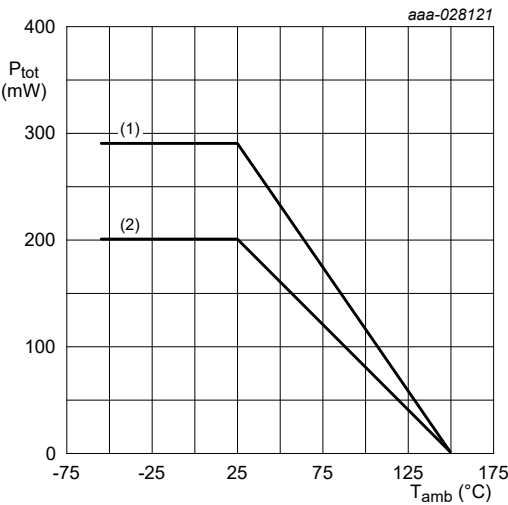
(1) FFR4 PCB, single-sided copper; 1 cm 2 (2) FR4 PCB, single-sided copper; standard footprint
