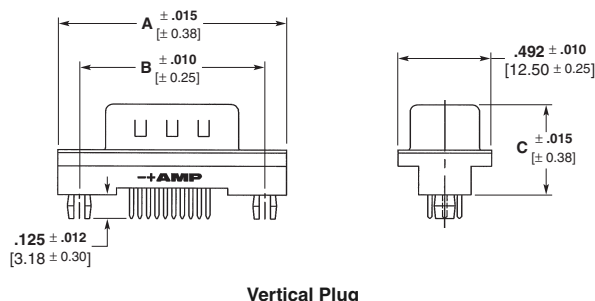
Vertical Plug
