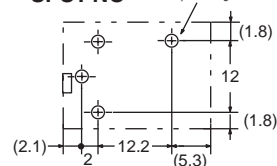
SPST-NO
