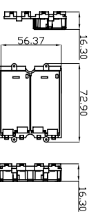
2X9V-BOX
