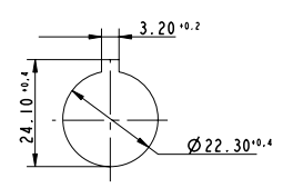
Panel cut-out to IEC 60947-5-1
