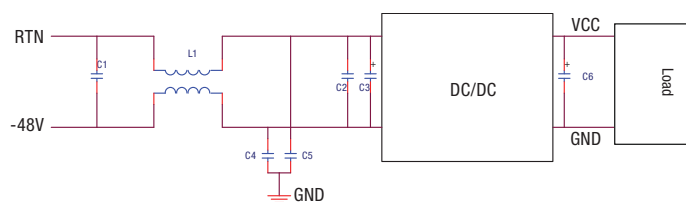
Figure 4. Conducted Emissions Test Circuit
